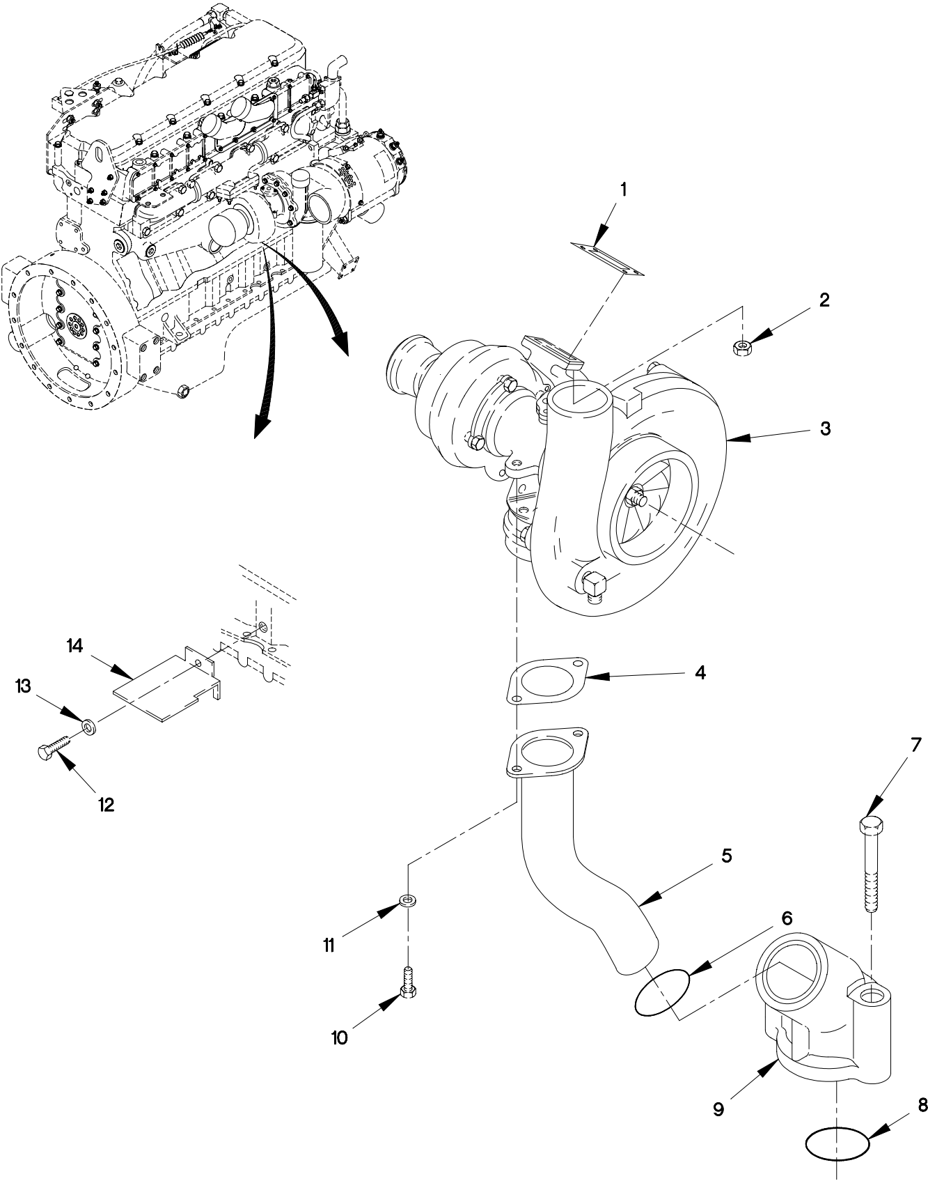
FIGURE 27. TURBOCHARGER
