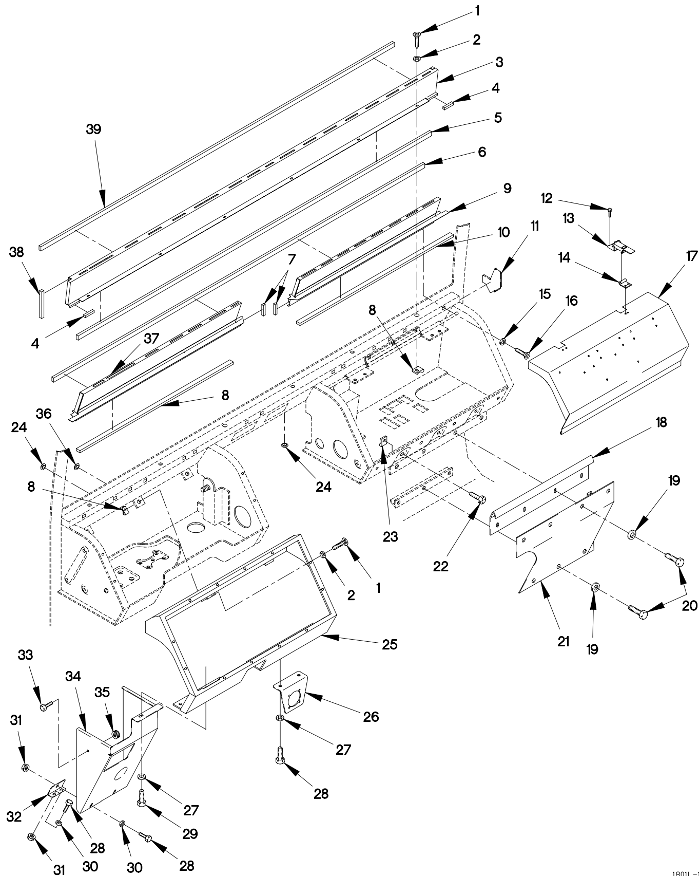
FIGURE 185. DASHBOARD
