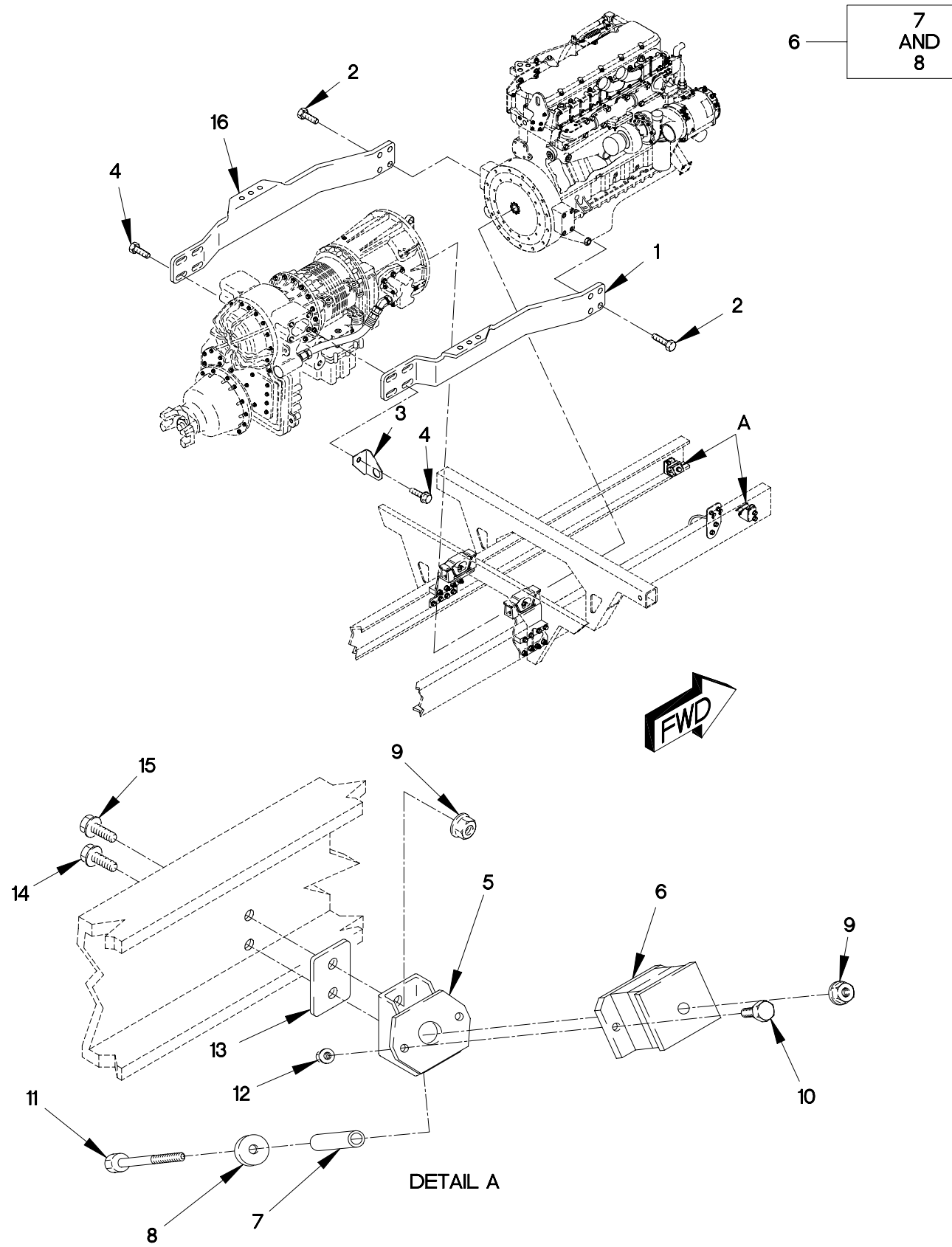
FIGURE 2. ENGINE MOUNTS
