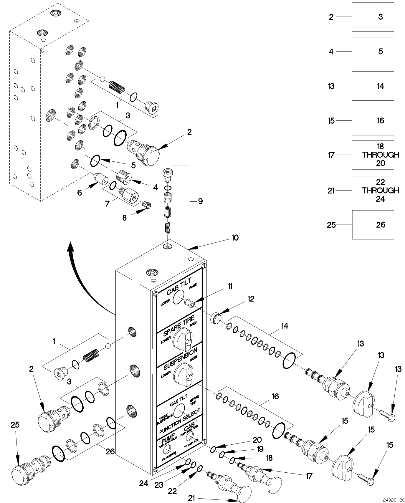
FIGURE 257. HYDRAULIC MANIFOLD ASSEMBLY
