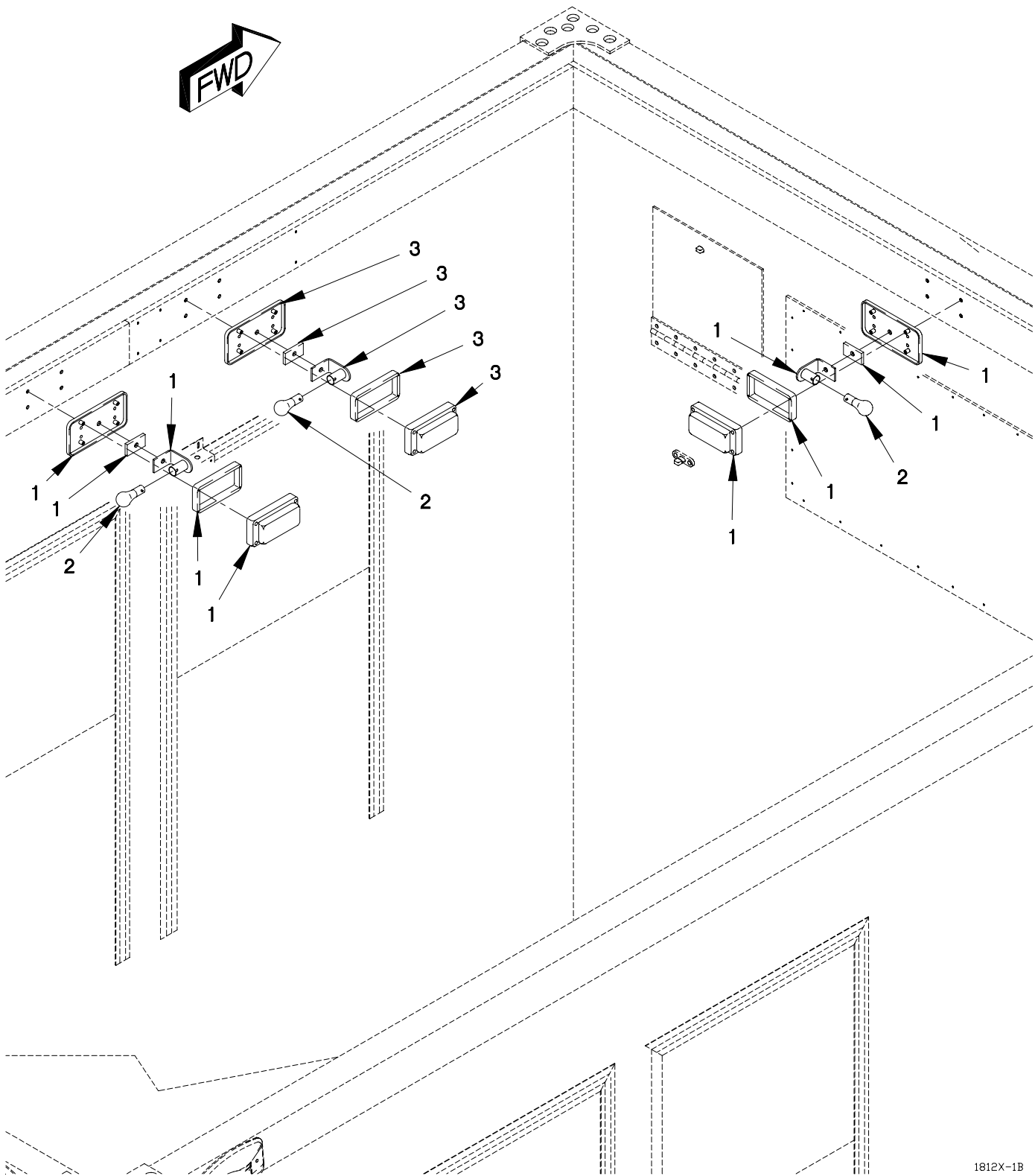
FIGURE 233. VAN BLACKOUT AND EMERGENCY LIGHTS
