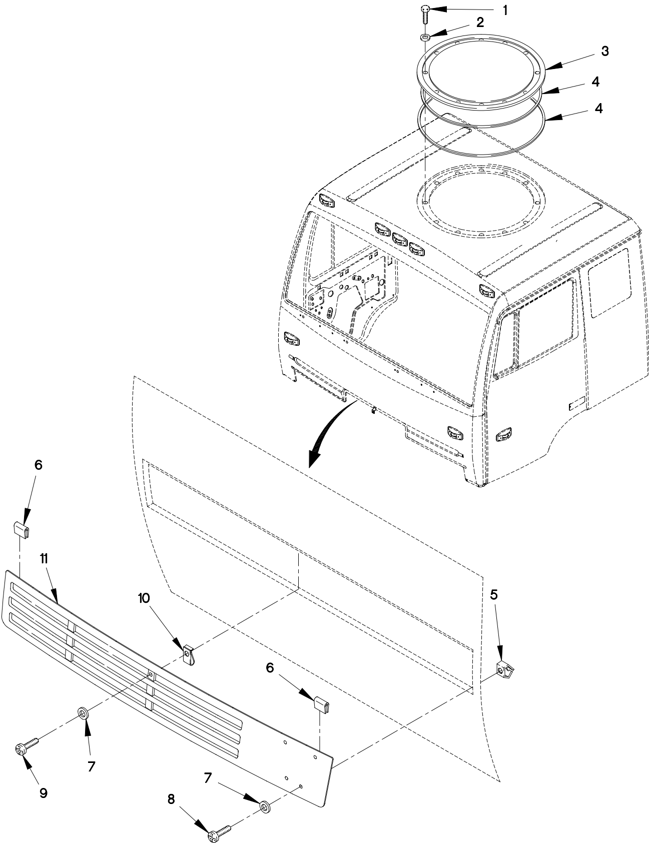
FIGURE 186. ROOF HATCH AND FRONT GRILL
