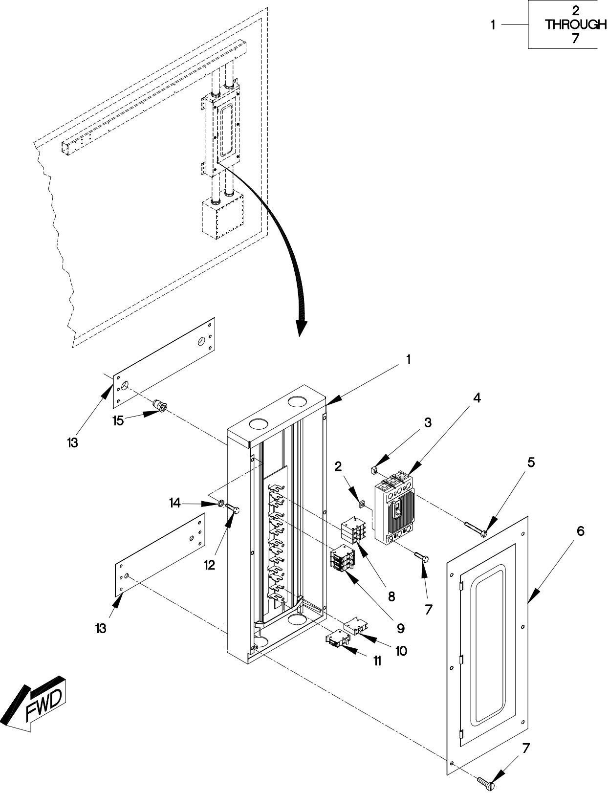
FIGURE 237. VAN BREAKER BOX ASSEMBLY
