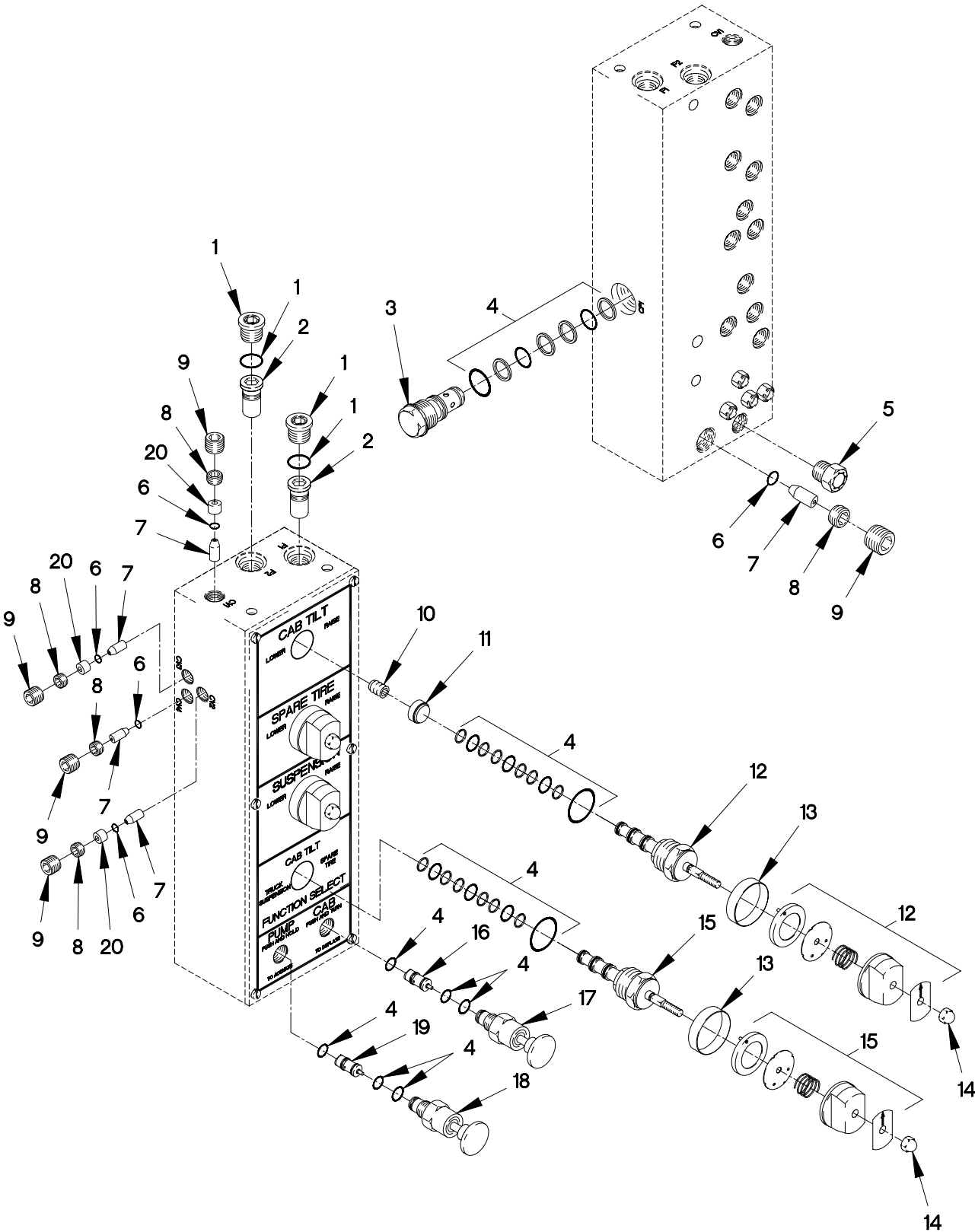
FIGURE 256. HYDRAULIC MANIFOLD ASSEMBLY
