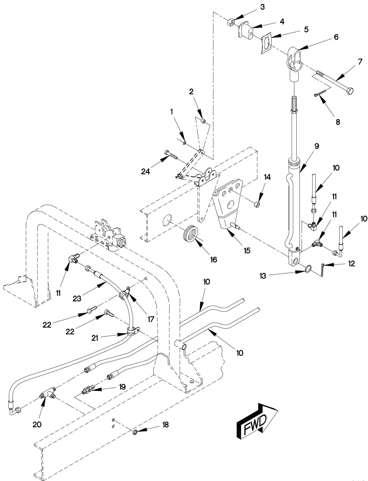
FIGURE 259. CAB HYDRAULIC CYLINDER, HOSES AND FITTINGS
