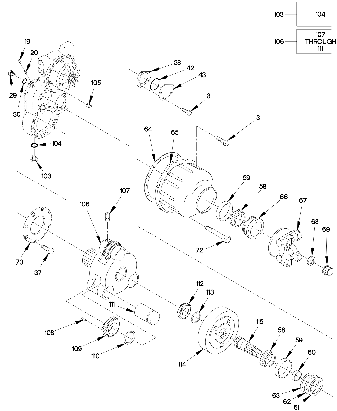
FIGURE 130. TRANSFER CASE MODULE (SHEET 4 OF 4)
