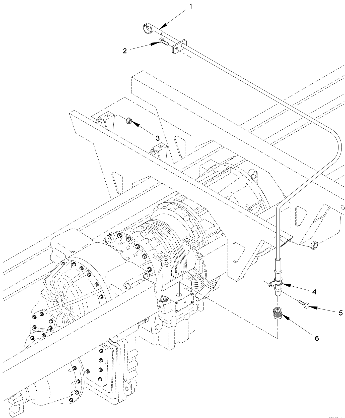
FIGURE 115. TRANSMISSION DIPSTICK
