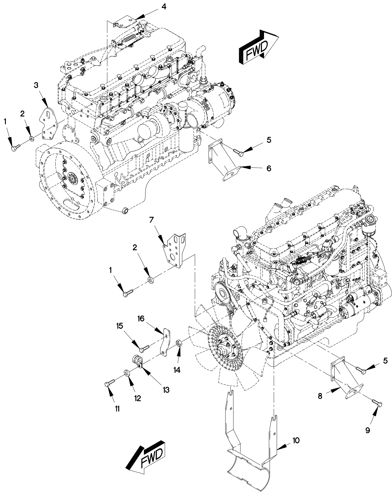
FIGURE 3. ENGINE BRACKETS
