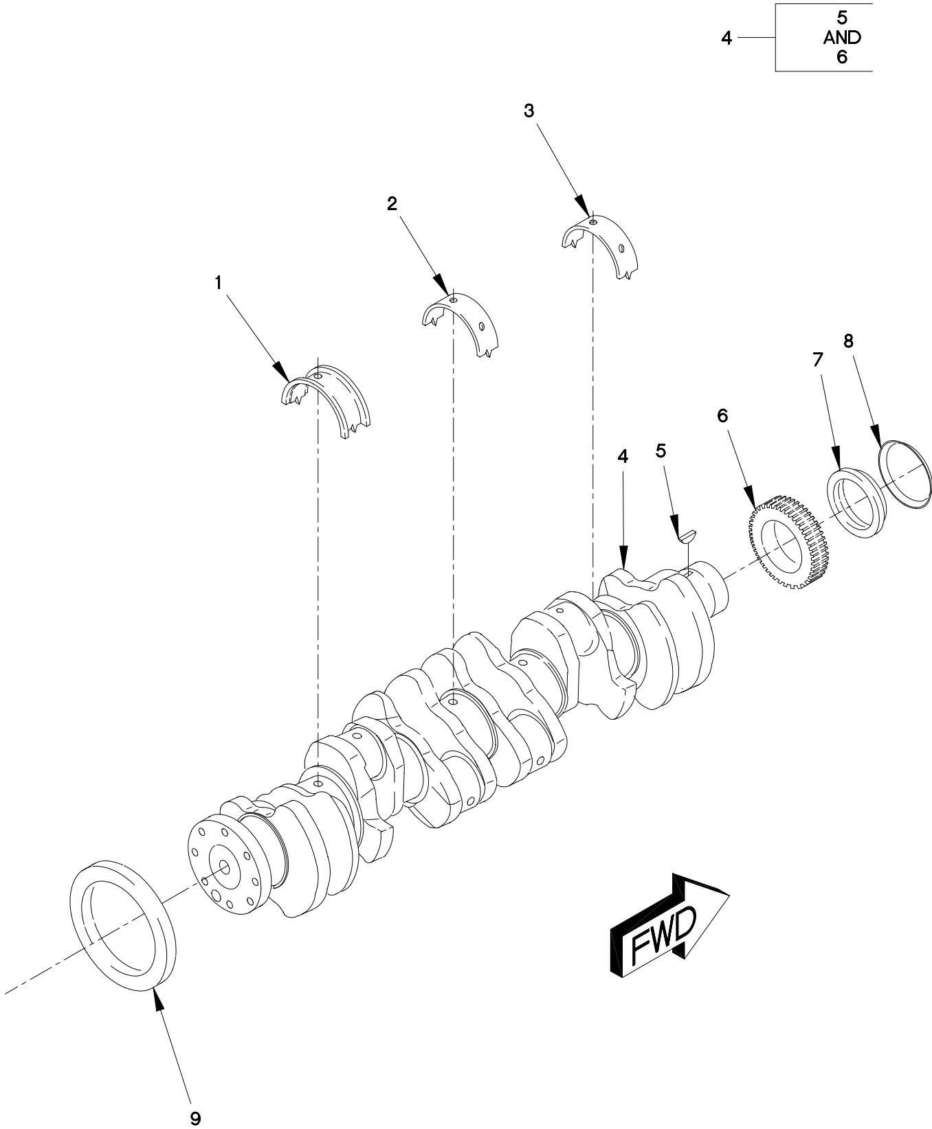
FIGURE 6. CRANKSHAFT
