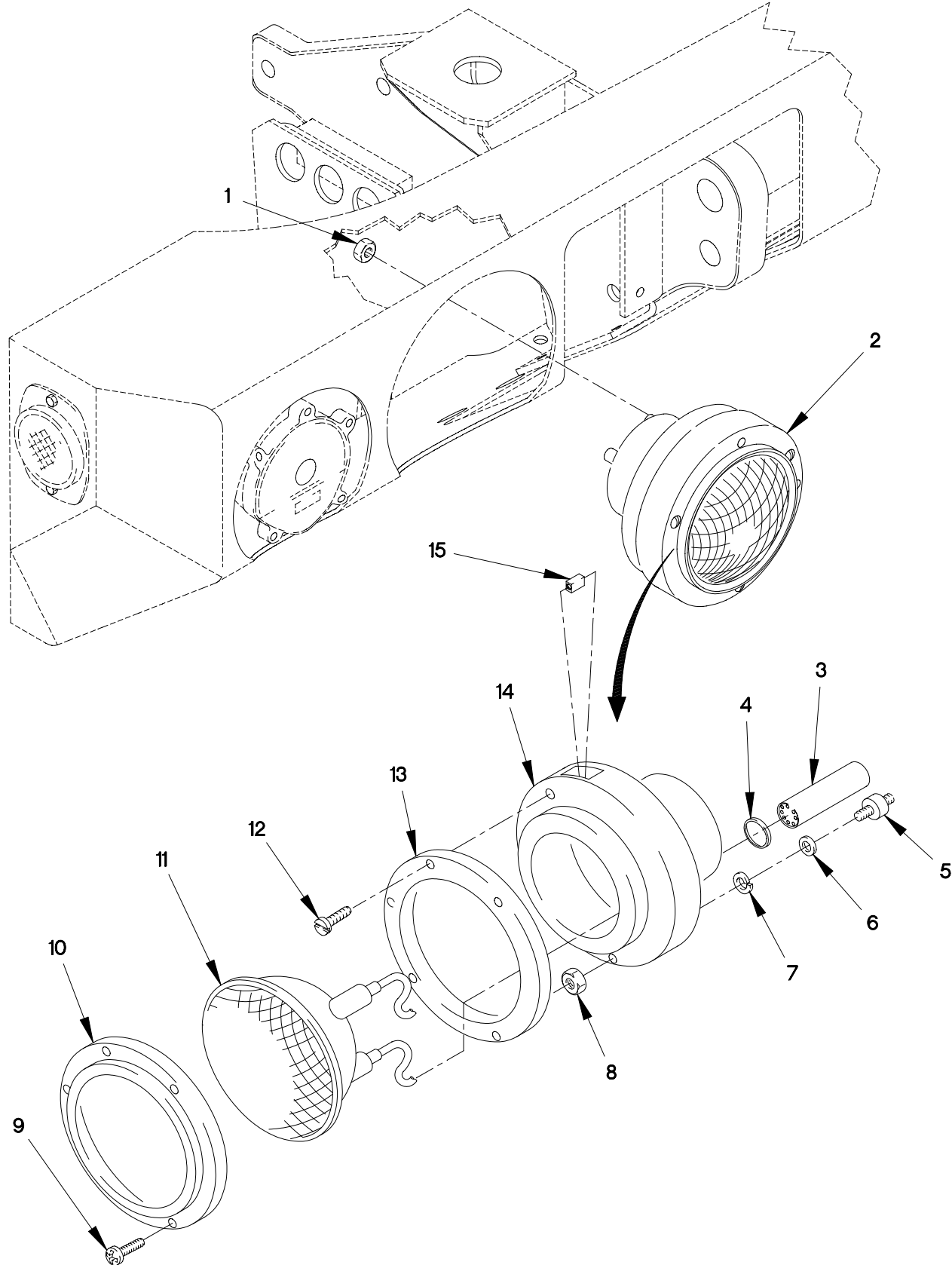
FIGURE 61. HEADLAMP ASSEMBLY
