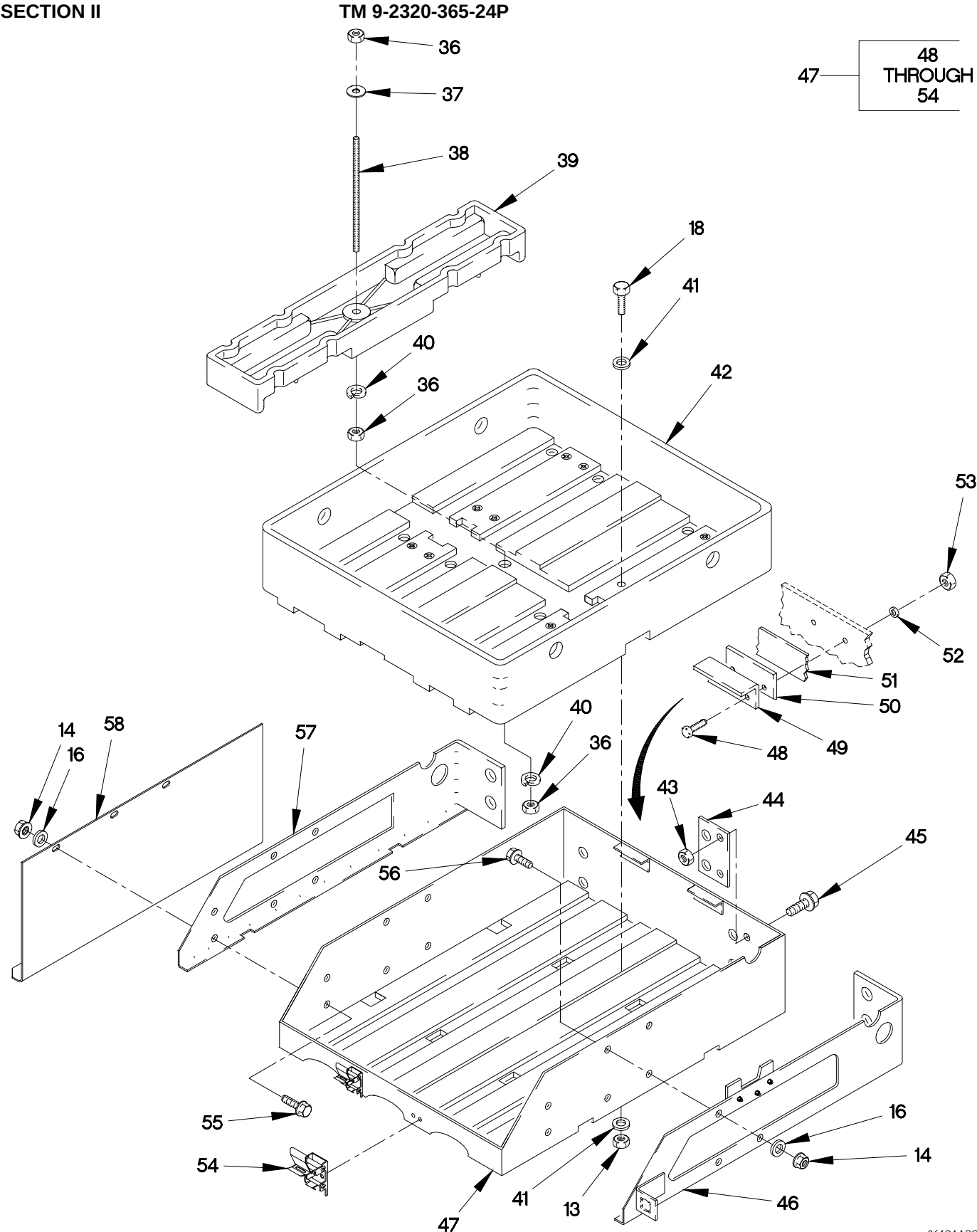
FIGURE 71. BATTERIES, BOX, GUARD AND CABLES (SHEET 2 OF 3)
