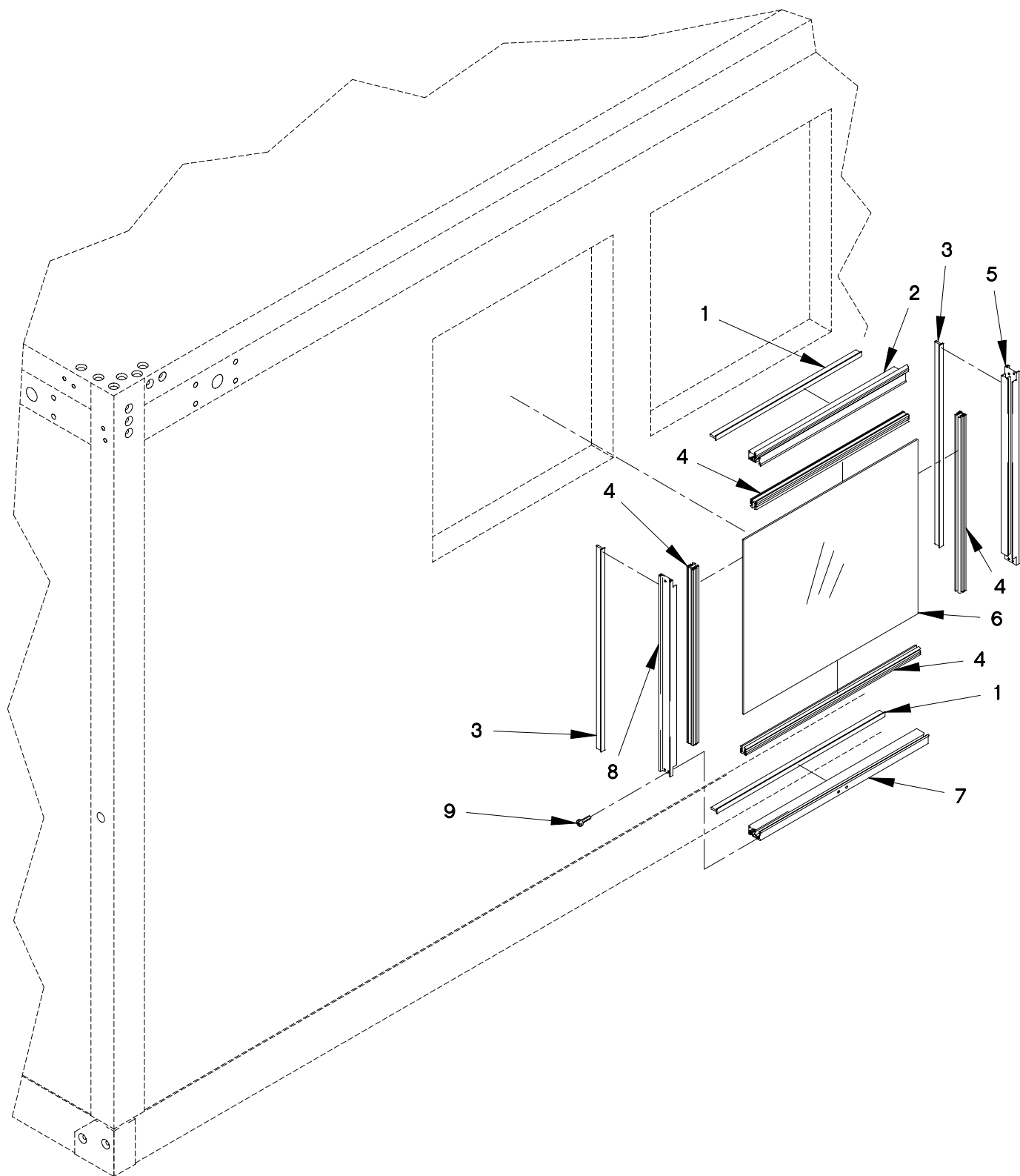
FIGURE 227. VAN LARGE WINDOW ASSEMBLY (SHEET 1 OF 3)
