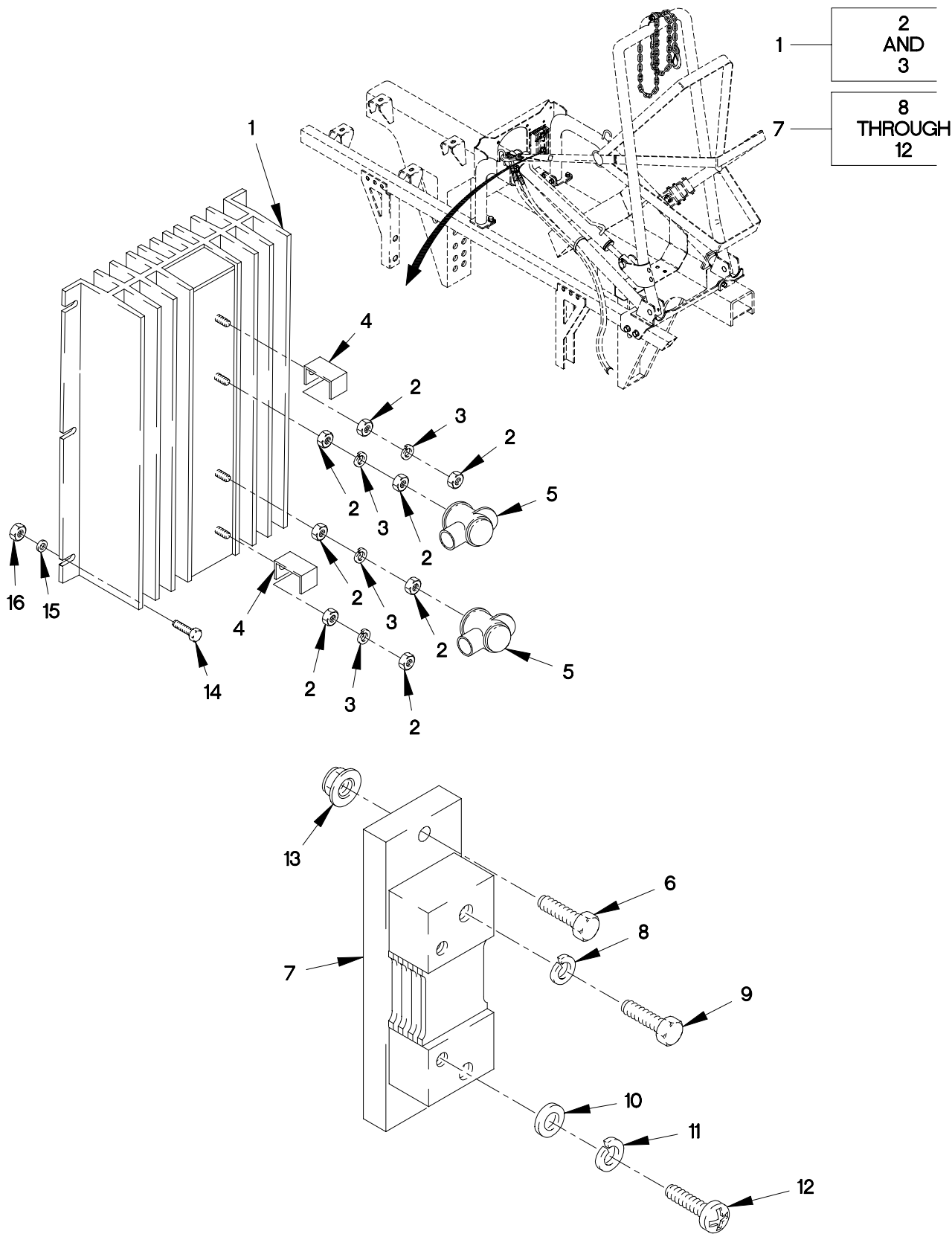
FIGURE 60. 100 AMP REVERSE POLARITY RELAY AND STARTER SHUNT
