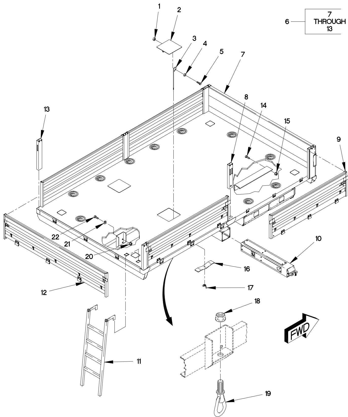
FIGURE 210. M1081 CARGO BED, DROPSIDE ASSEMBLY AND LADDER
