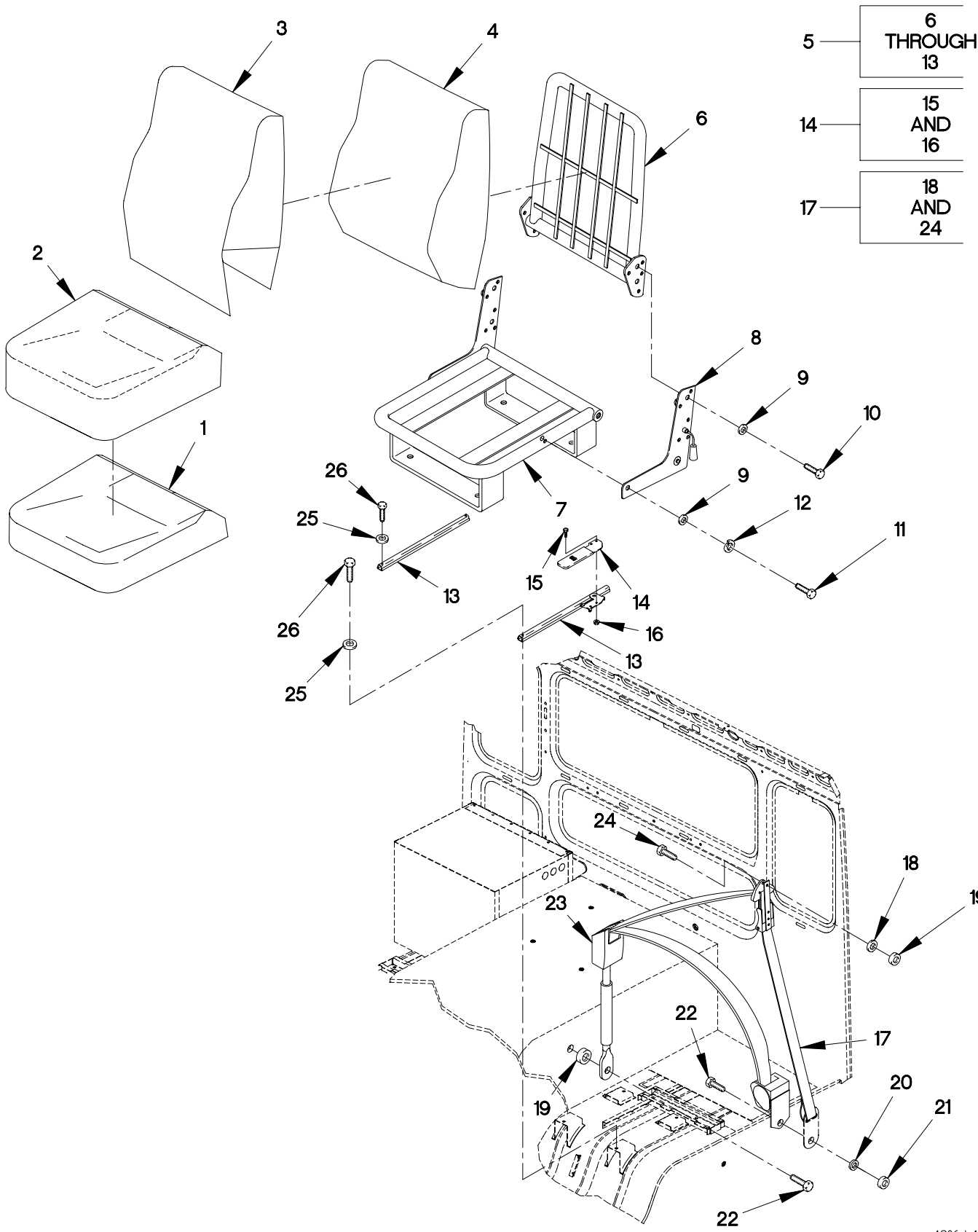
FIGURE 206. DRIVER SEAT AND SEAT BELT
