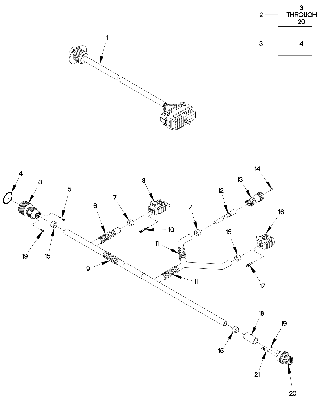
FIGURE 77. TRANSMISSION HARNESS
