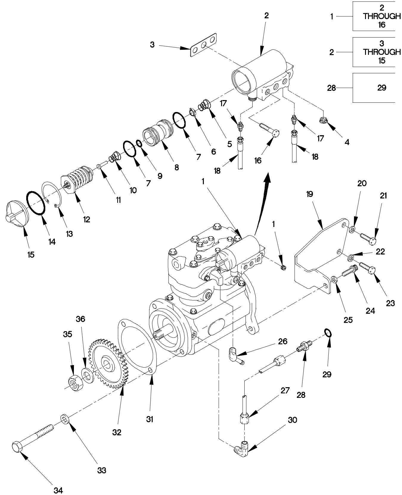
FIGURE 157. AIR COMPRESSOR
