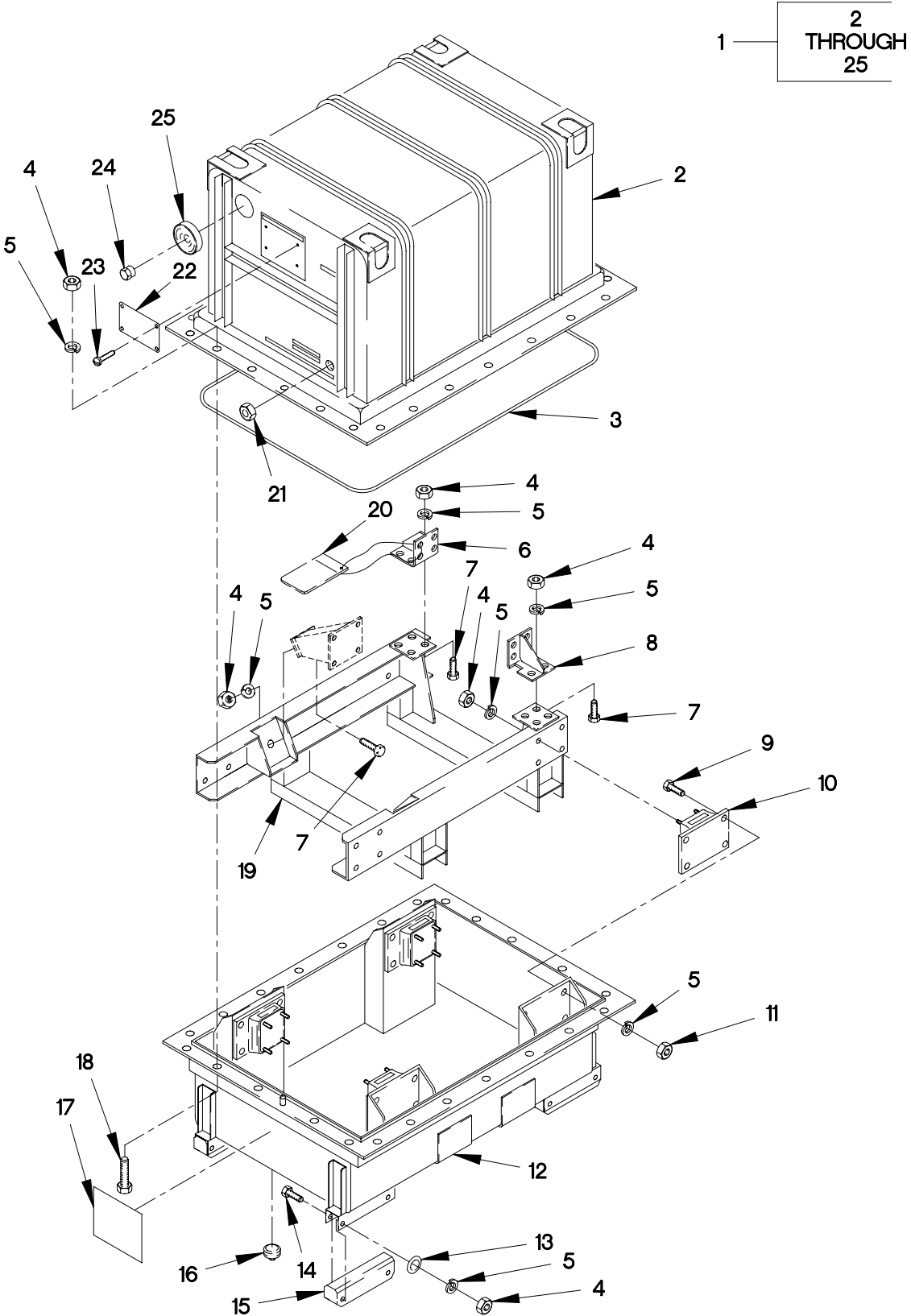
FIGURE 263. ENGINE CONTAINER
