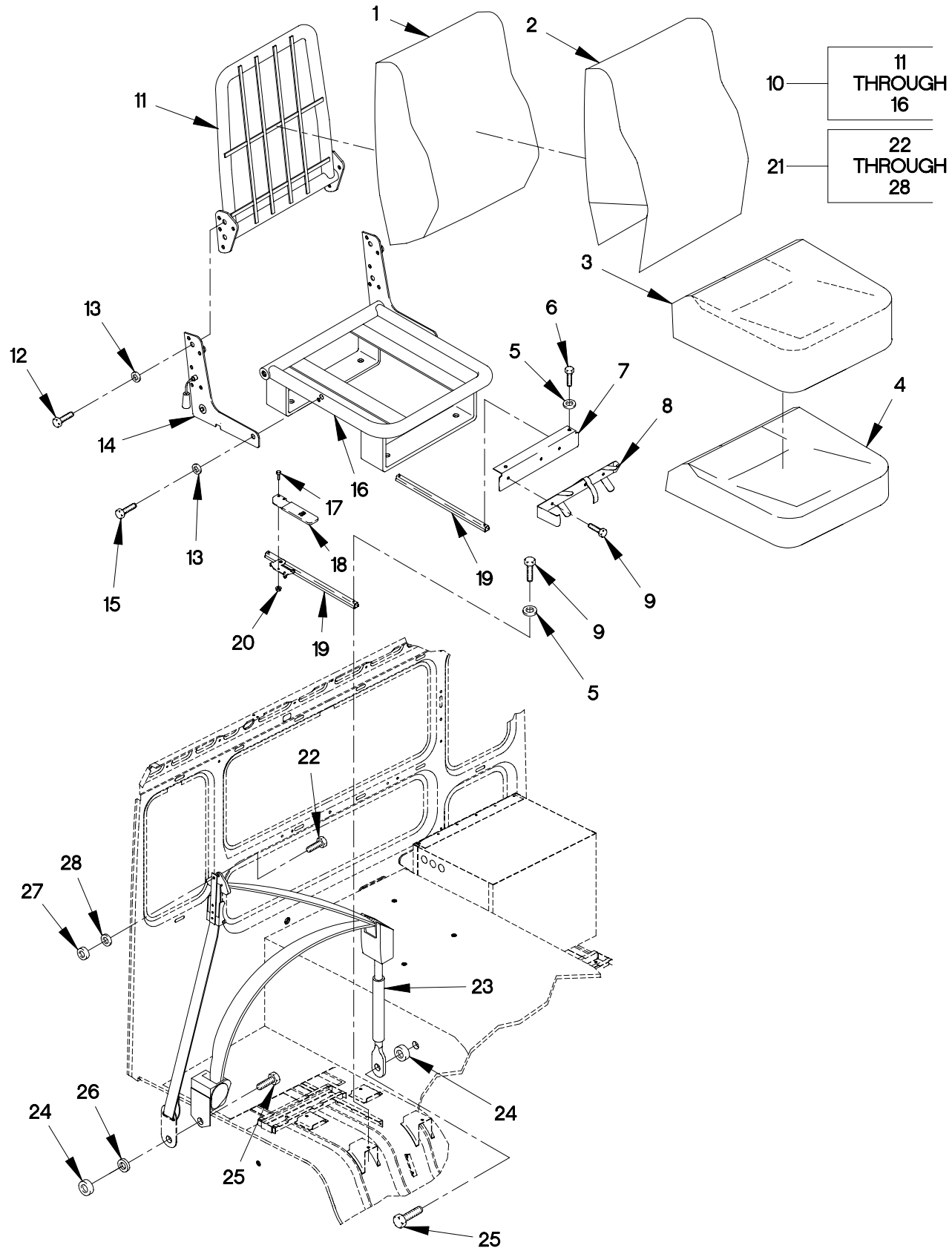
FIGURE 205. PASSENGER SEAT AND SEAT BELT
