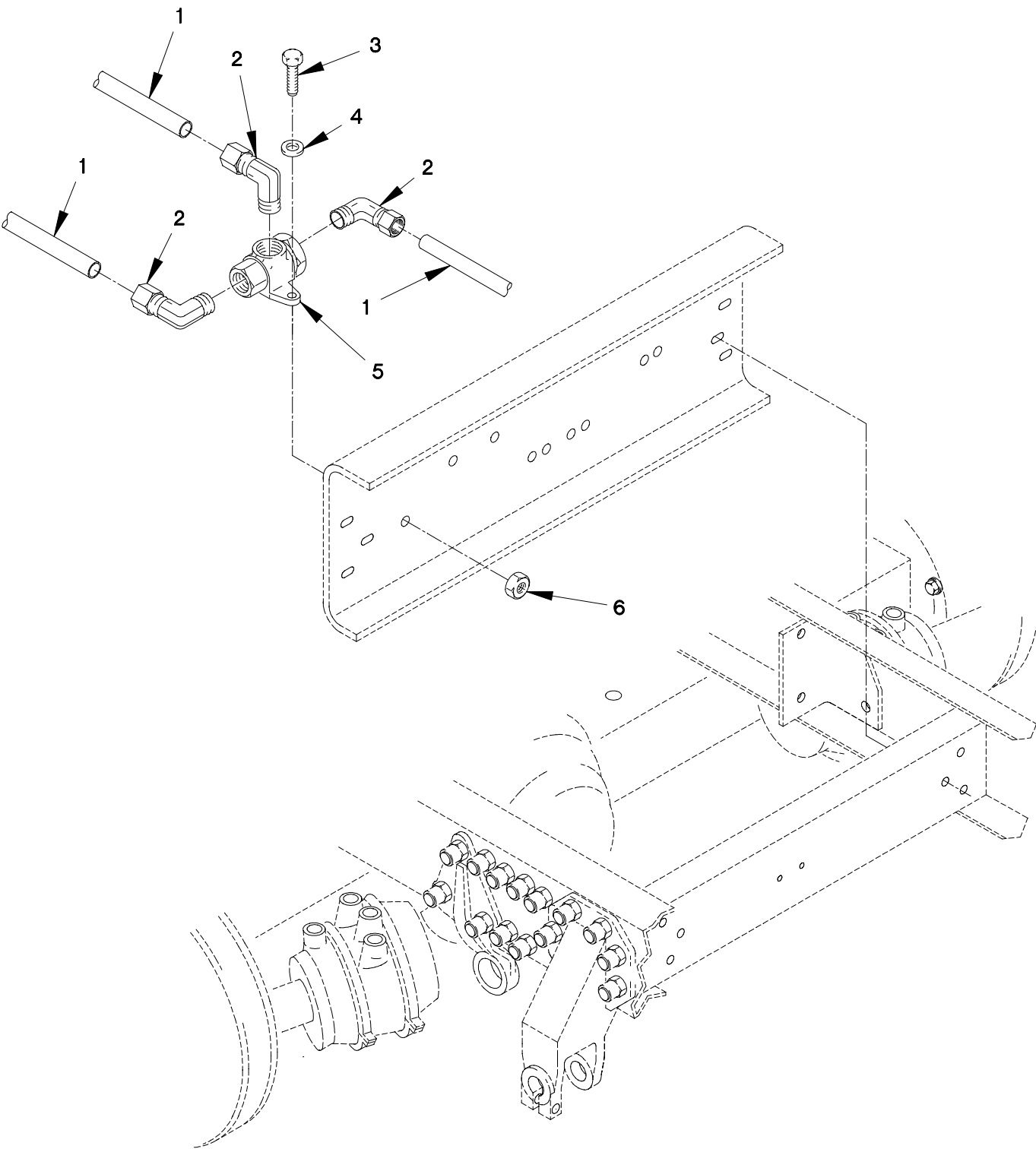
FIGURE 147. TWO WAY CHECK VALVE, HOSES AND FITTINGS
