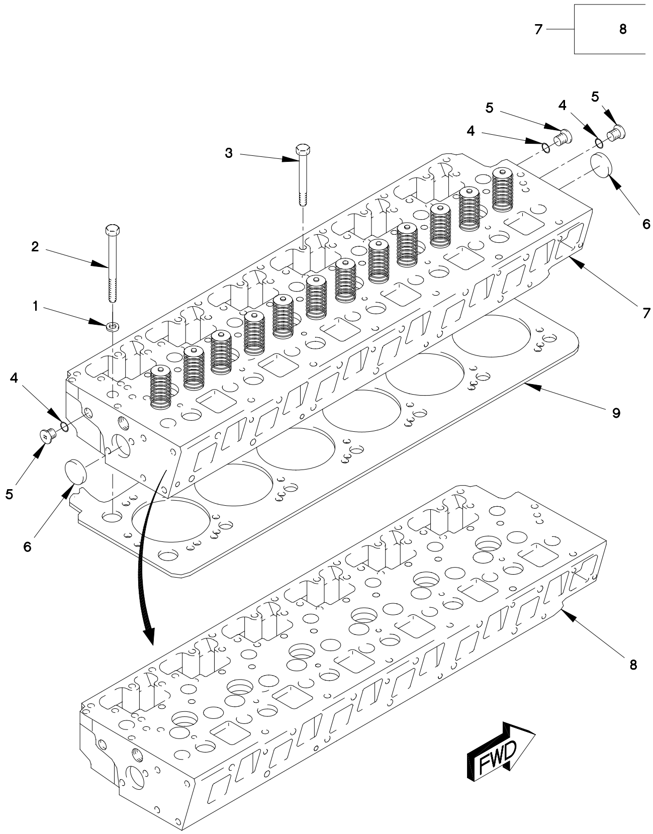
FIGURE 4. CYLINDER HEAD WITH VALVES AND GASKET
