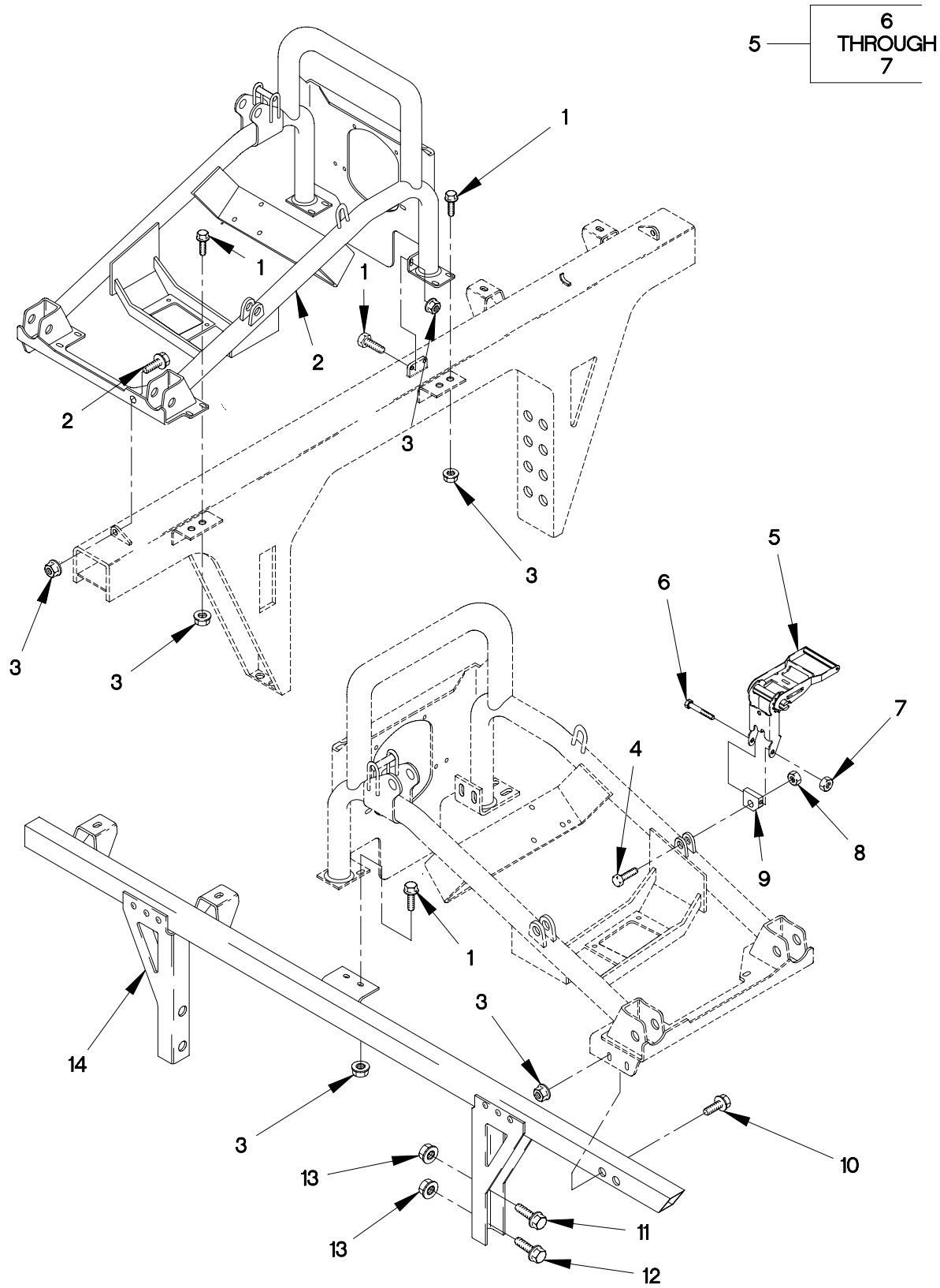
FIGURE 175. SPARE TIRE RETAINER (SHEET 1 OF 3)
