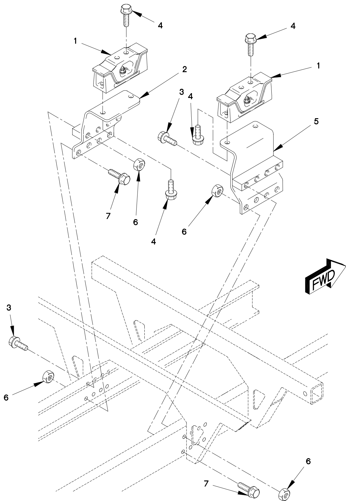
FIGURE 114. TRANSMISSION MOUNTS
