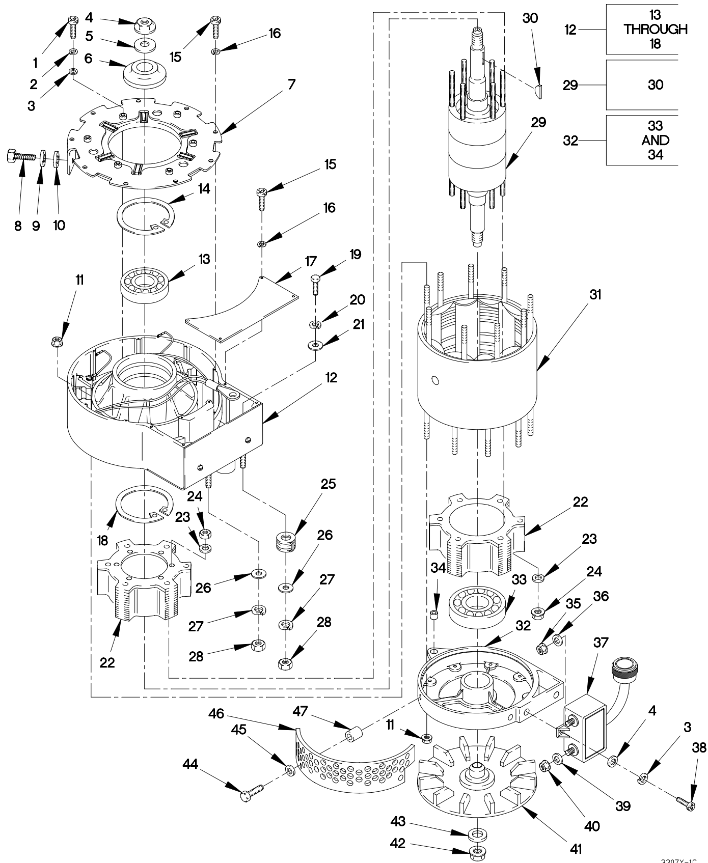
FIGURE 274. 200A ALTERNATOR AND REGULATOR
