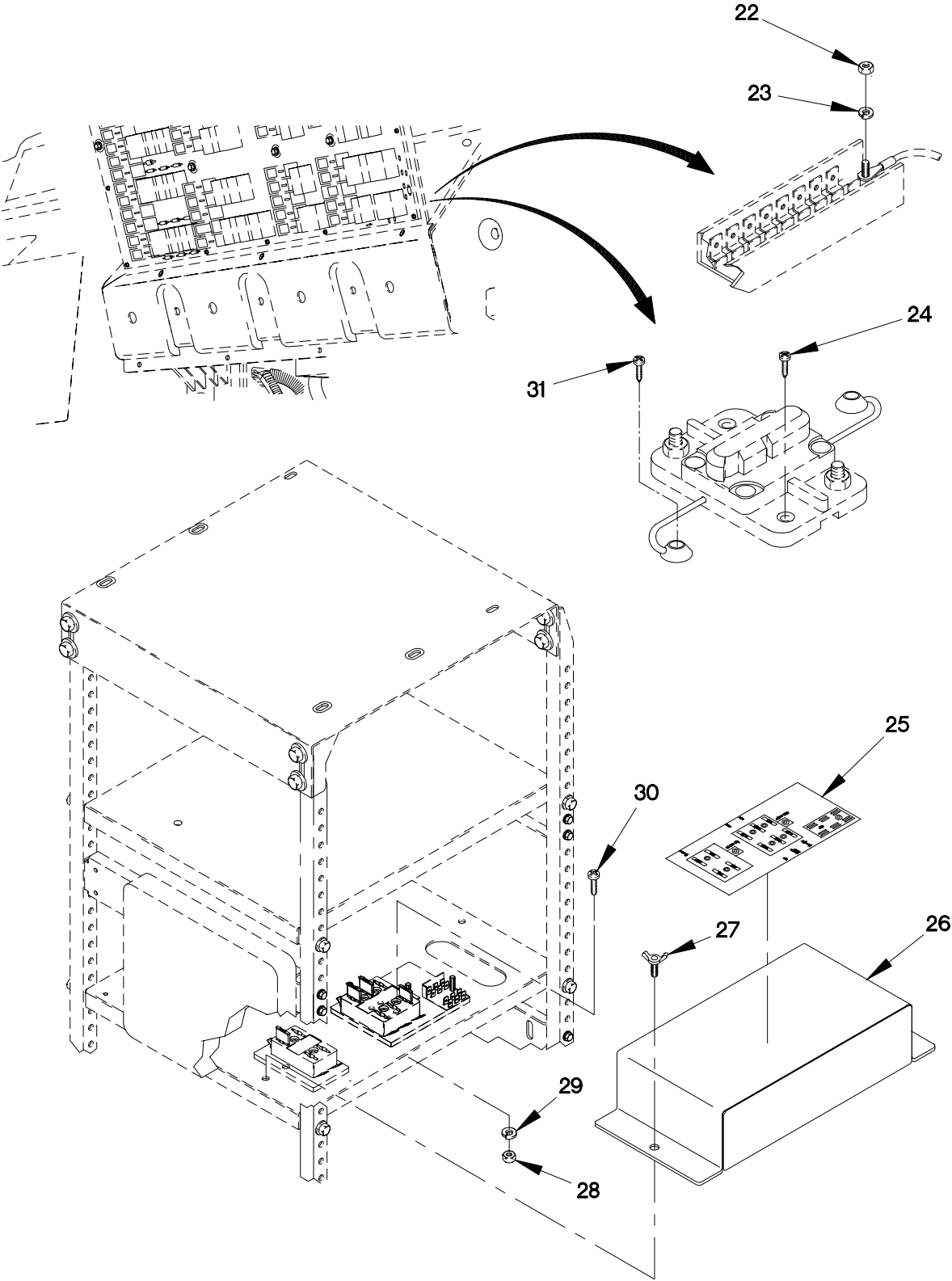
FIGURE 289. DIGITIZATION ELECTRICAL KIT (SHEET 2 OF 2)
