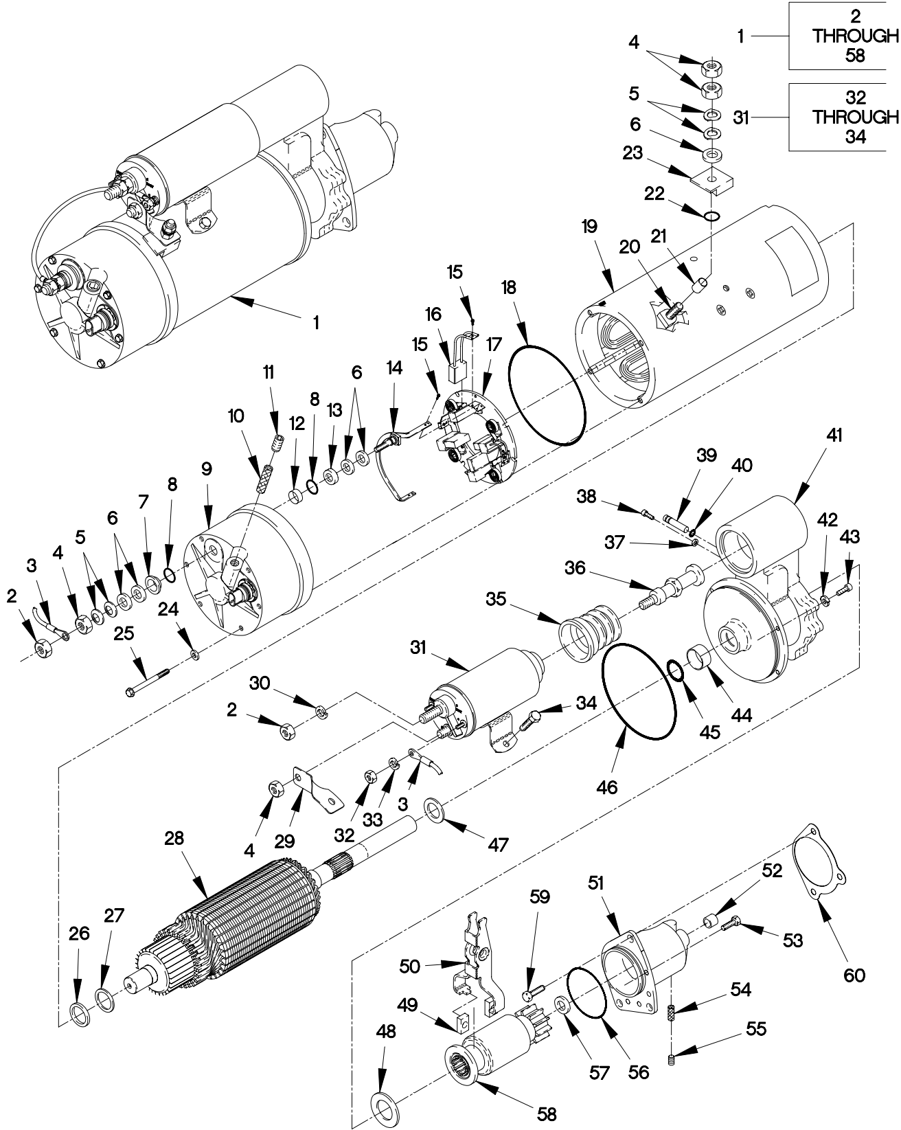
FIGURE 49. M0017703ME STARTER AND SOLENOID
