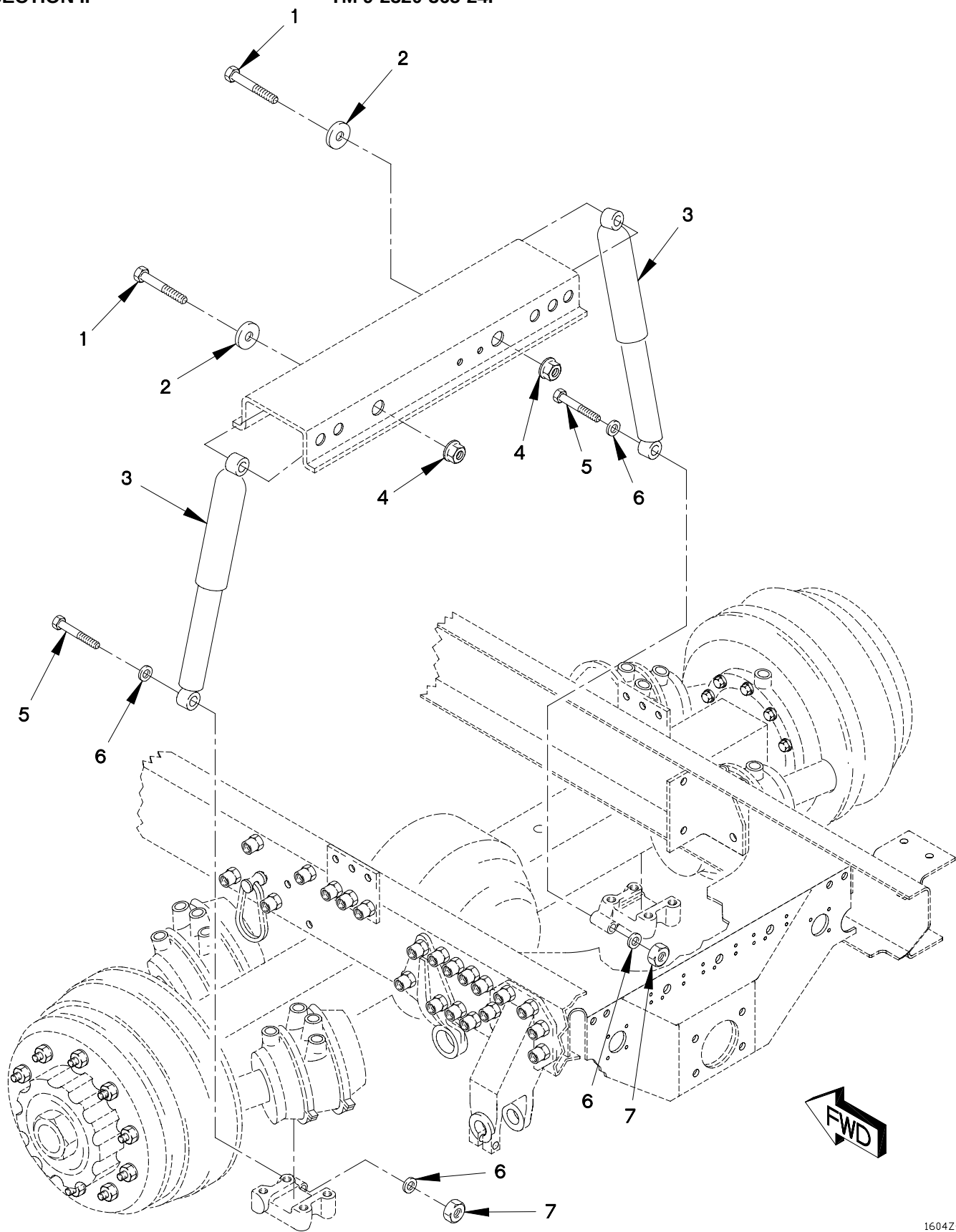
FIGURE 181. REAR SHOCKS
