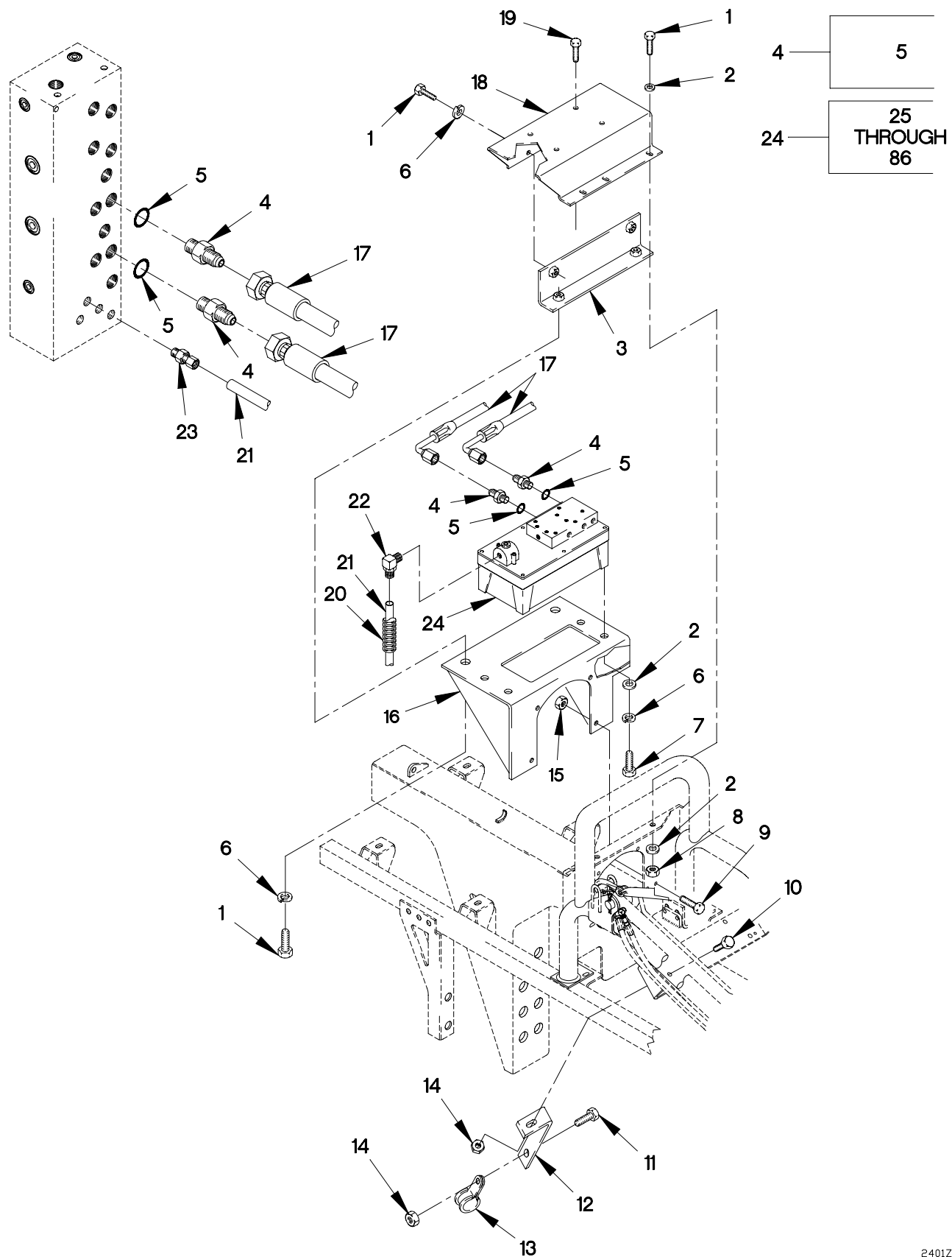
FIGURE 253. AIR/HYDRAULIC POWER UNIT, HOSES AND FITTINGS (SHEET 1 OF 2)
