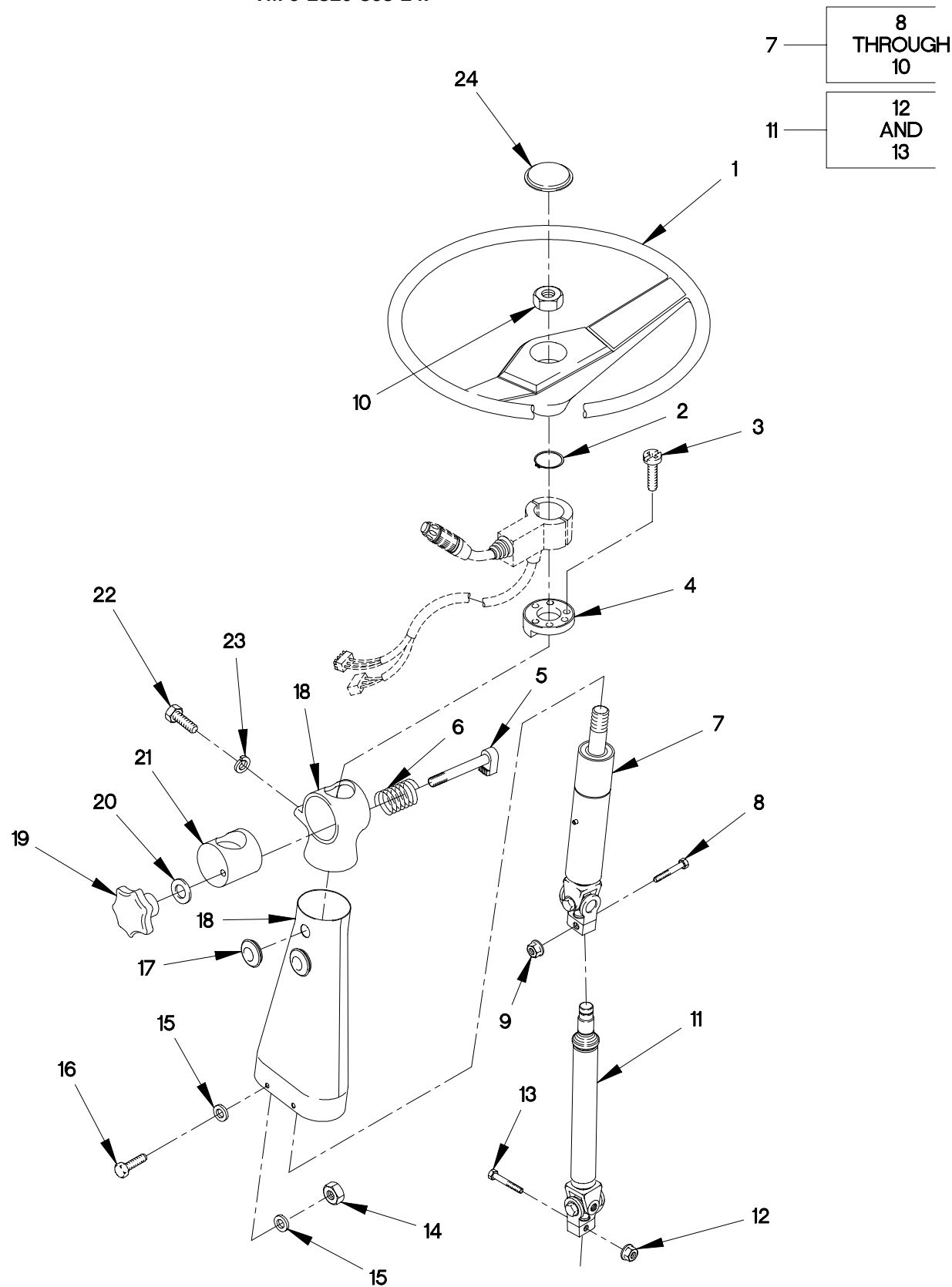
FIGURE 161. STEERING WHEEL AND COLUMN
