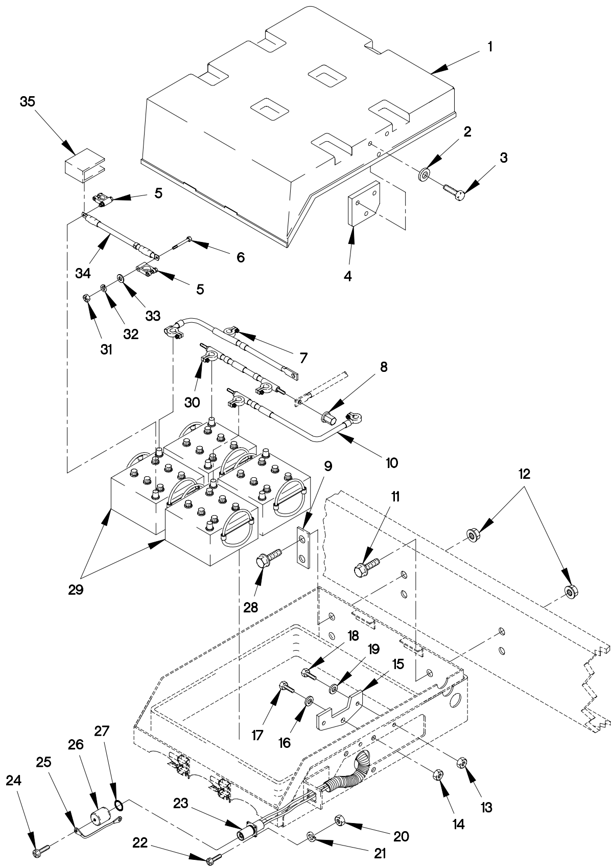
FIGURE 71. BATTERIES, BOX, GUARD AND CABLES (SHEET 1 OF 3)
